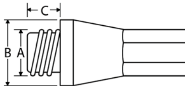
Detachable drill steel thread dimensions by type
